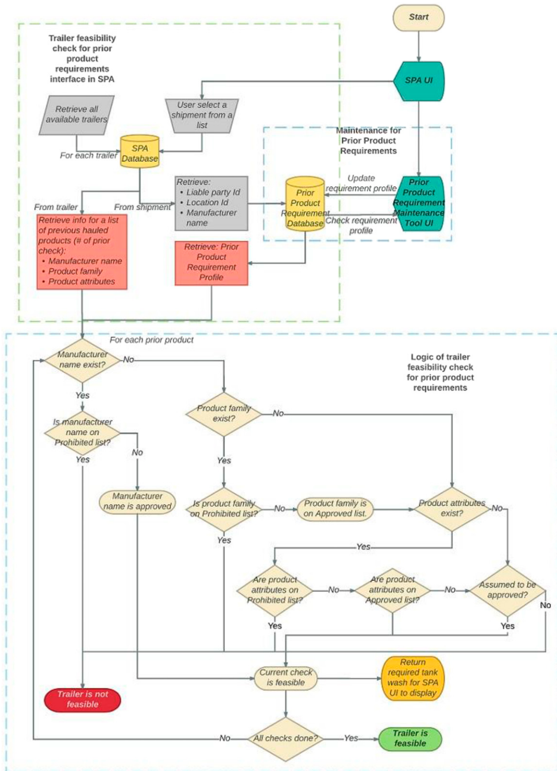
Figure 8. (Color online) The Logic Used to Validate Prior-Product Compatibility
