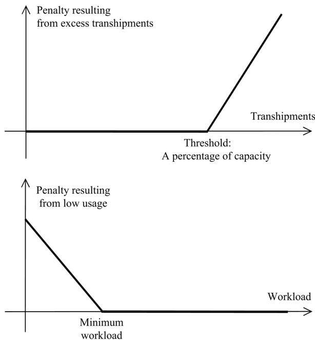
Figure 2: A laboratory that receives too few or too many samples to analyze incurs additional operational costs. When it receives too many samples, a penalty results from the excessive number of transshipments; however, when it receives too few samples, a penalty results from the inadequate use of installed capacity.
